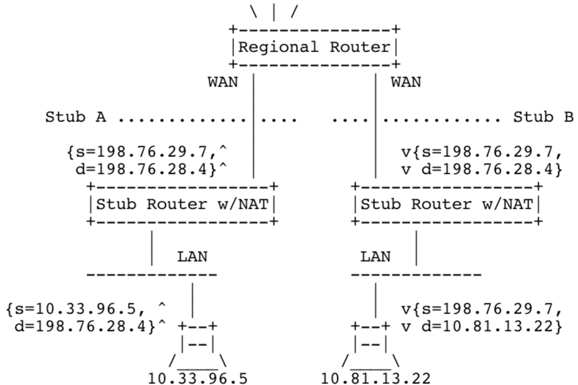
Figure 2: Basic NAT Operation
